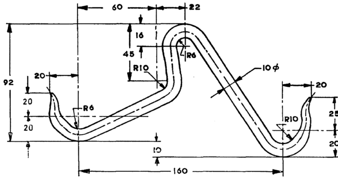
Figure 1 — Dimensions of gambrel for sheep and goats
