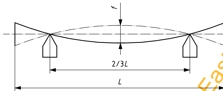
Figure A.1 — Determination of pipe straightness
