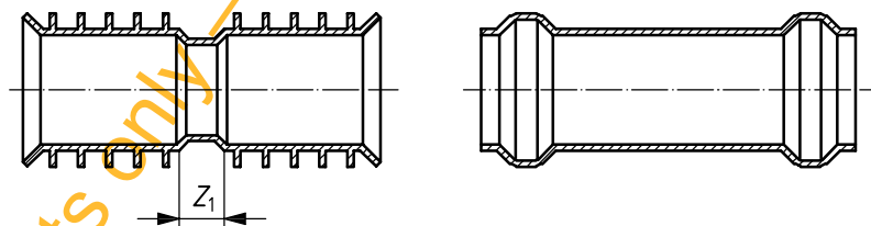
Figure 3 — Example of a coupler and slip coupler
