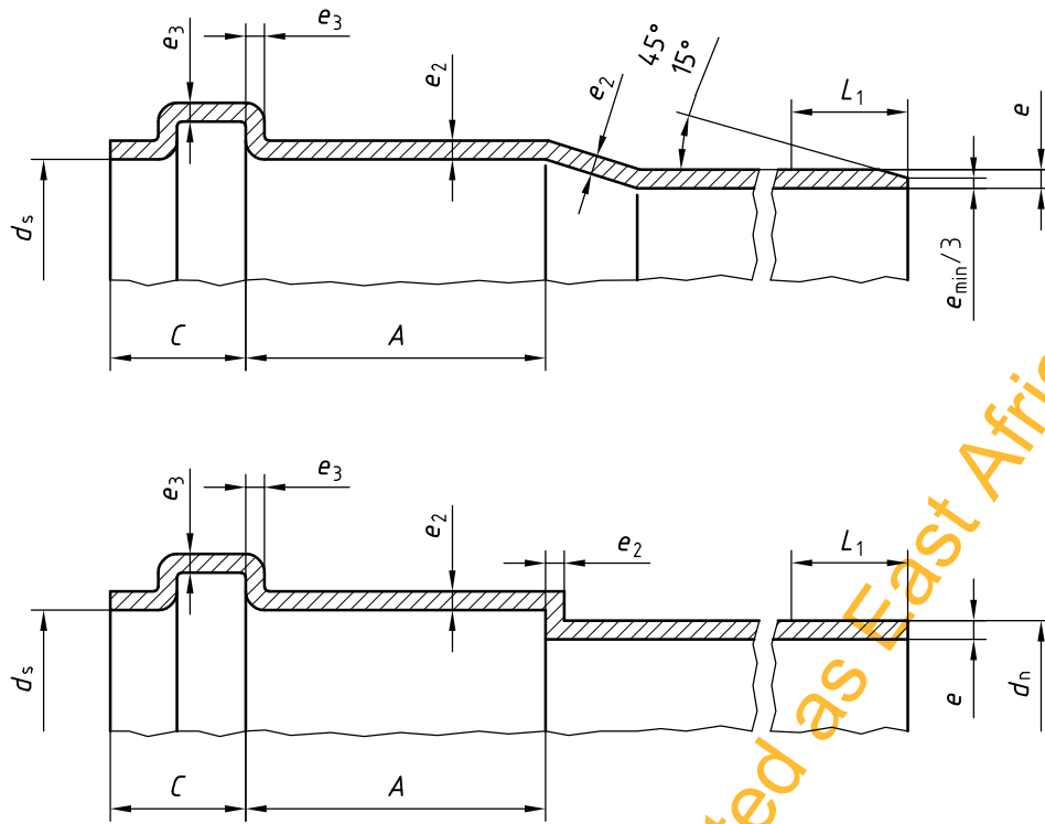
Figure 3 — Dimensions of sockets and spigot ends for ring seal joints
