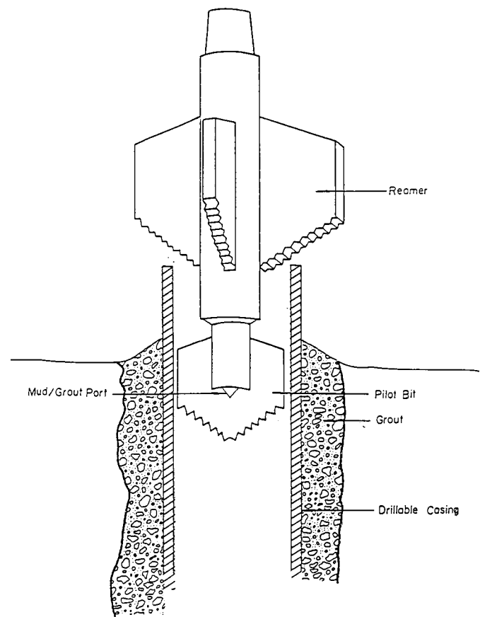
FIG. 3 Over Drilling by Mud Rotary Procedure
