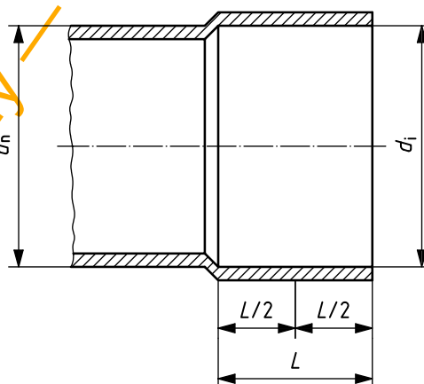
Figure 2 — Socket for solvent cementing
