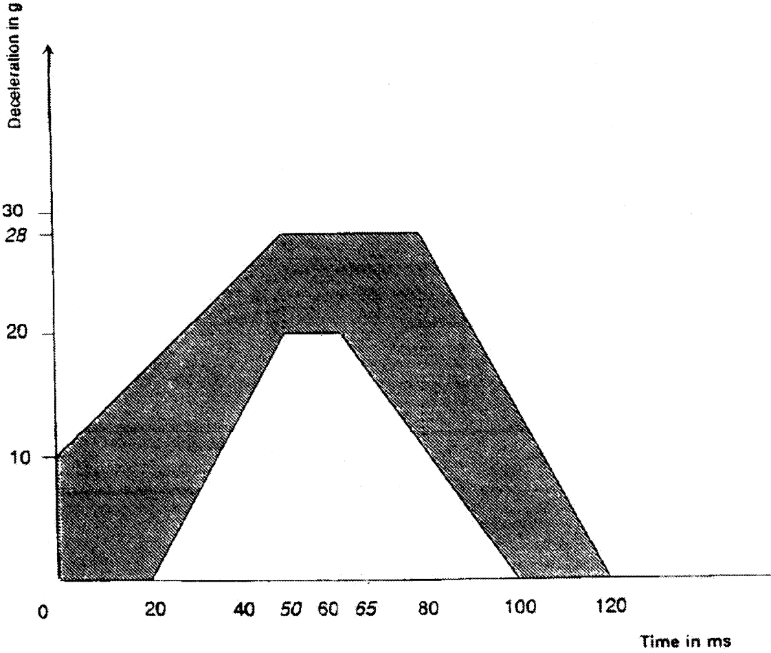
Sled declaration corridor as a function of time (Frontal impact)
