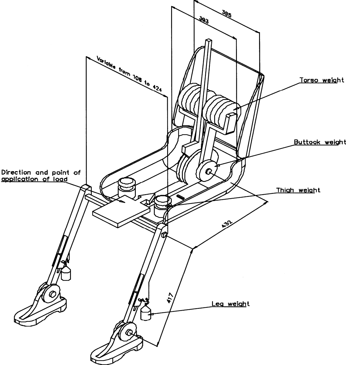
Figure 2 — Dimensions of the 3-D H machine elements and load distribution (Dimensions in millimeters)
