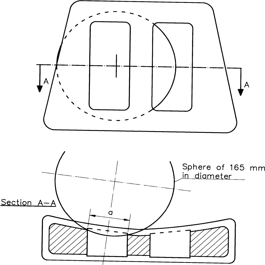
Figure 2 — Example of vertical gaps
