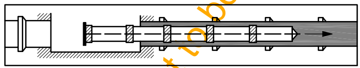
b) Installation by pulling
